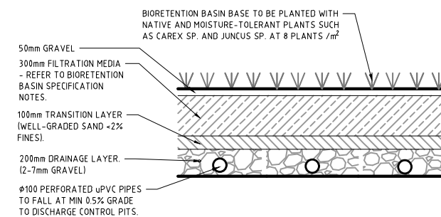
BIORETENTION FILTER MEDIA DETAIL
