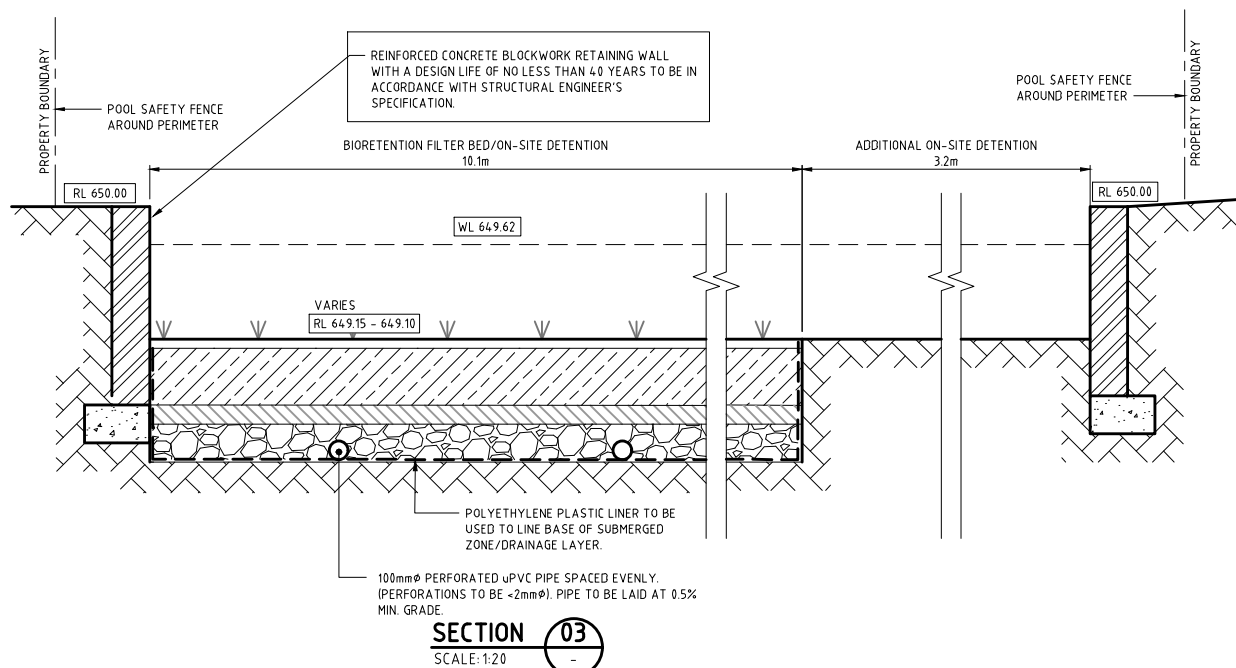
SECTION 03 SCALE: 1:20 BIORETENTION BASIN / ON-SITE DETENTION (OSD) TYPICAL SECTION
