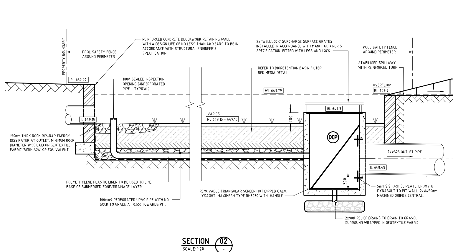
SECTION 02 SCALE: 1:20 BIORETENTION BASIN / ON-SITE DETENTION DETAIL
