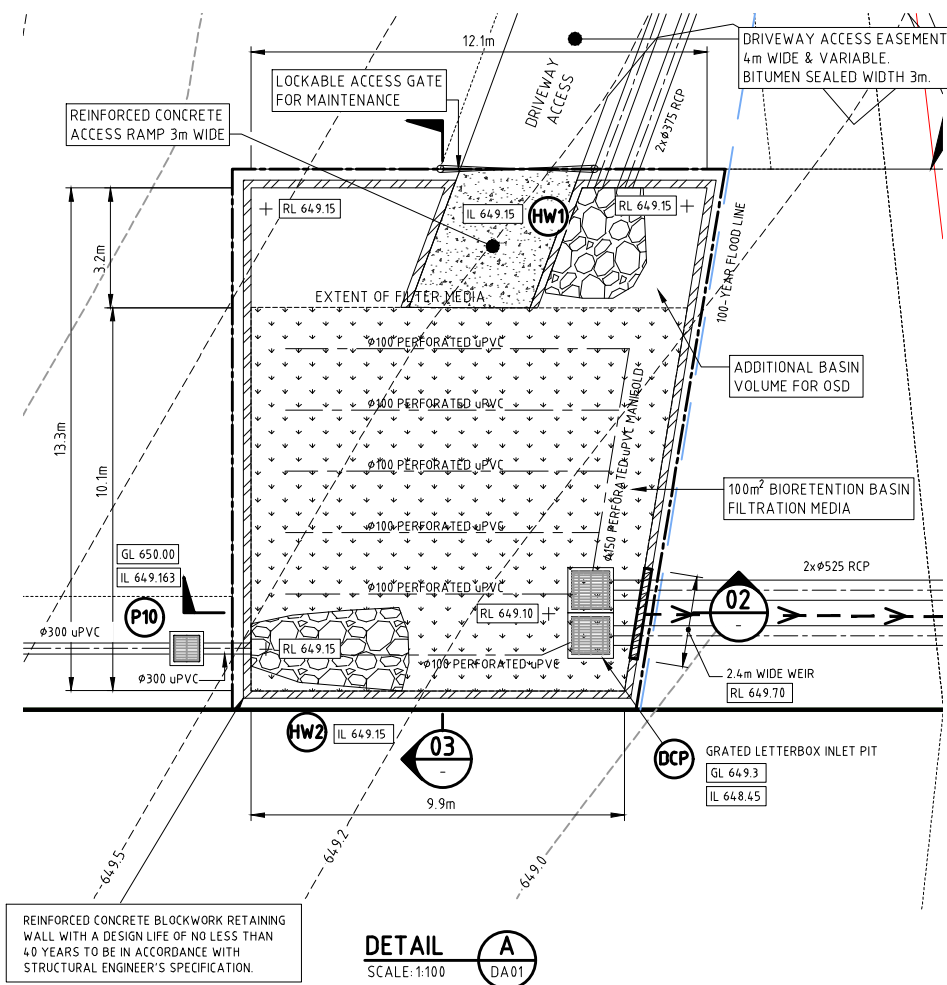
BIORETENTION BASIN / ON-SITE DETENTION (OSD) DETAIL
