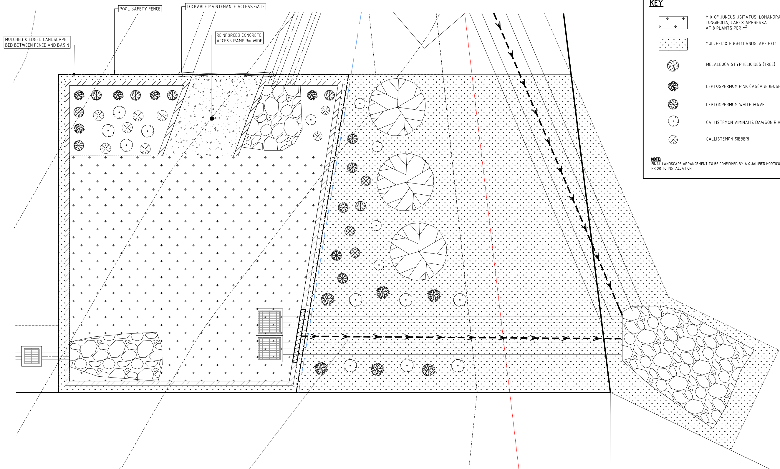
BIORETENTION BASIN LANDSCAPE PLAN
