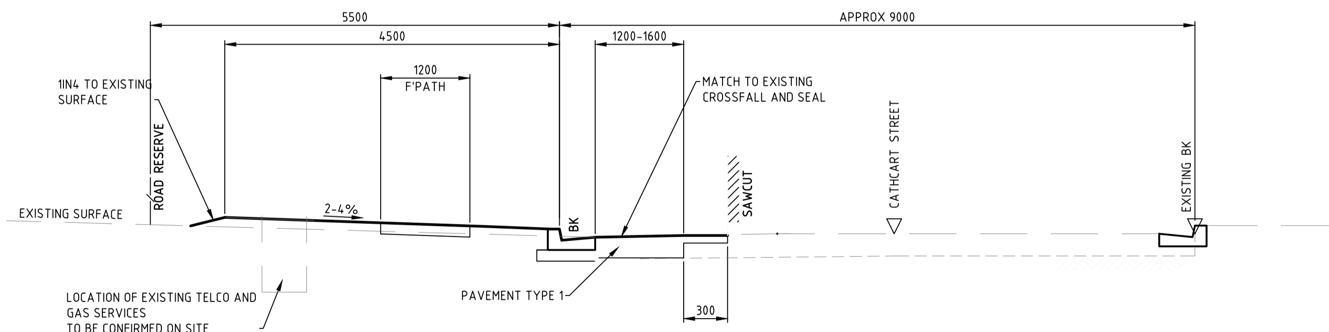
CATHCART STREET WIDENING TYPICAL SECTION SCALE 1:50
