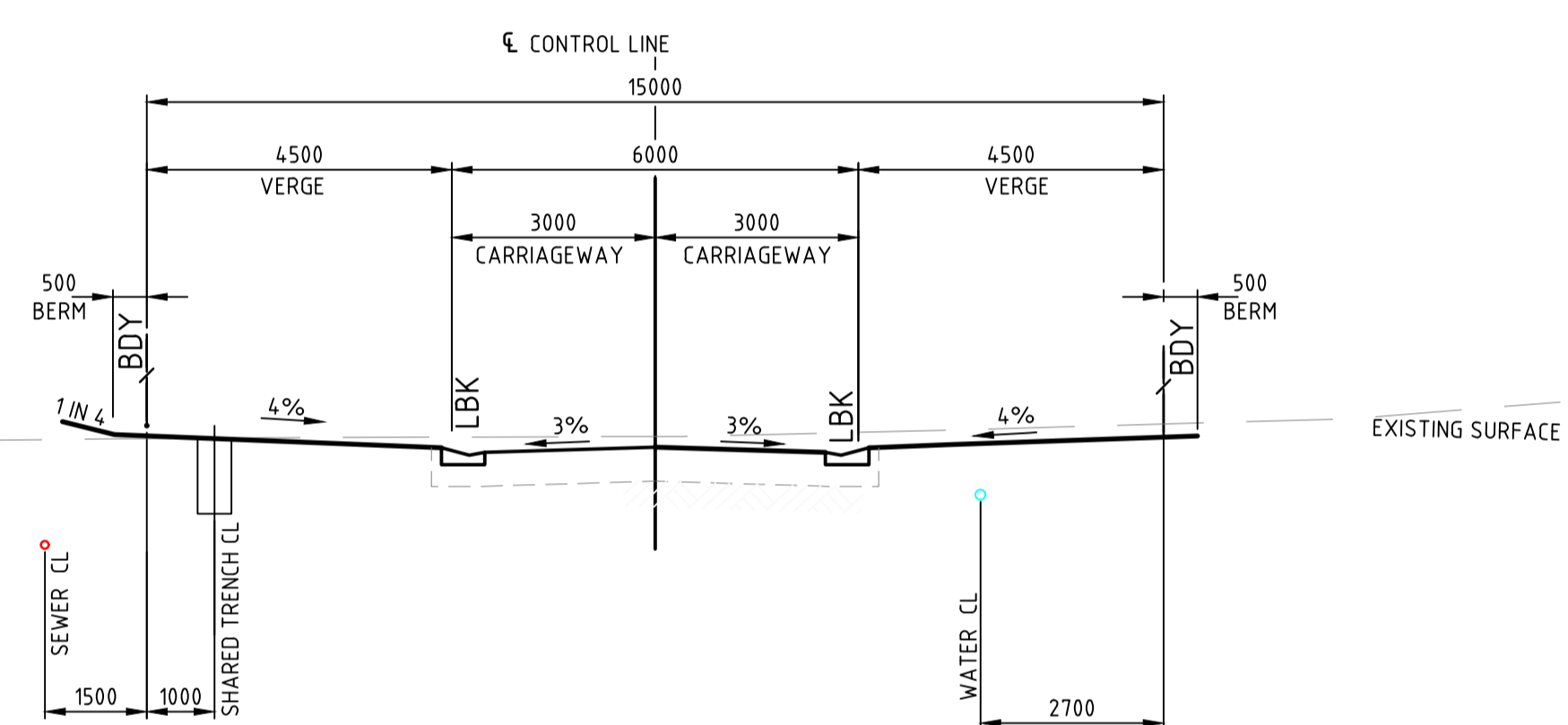
ROAD 01 - TYPICAL SECTION SCALE 1:100
